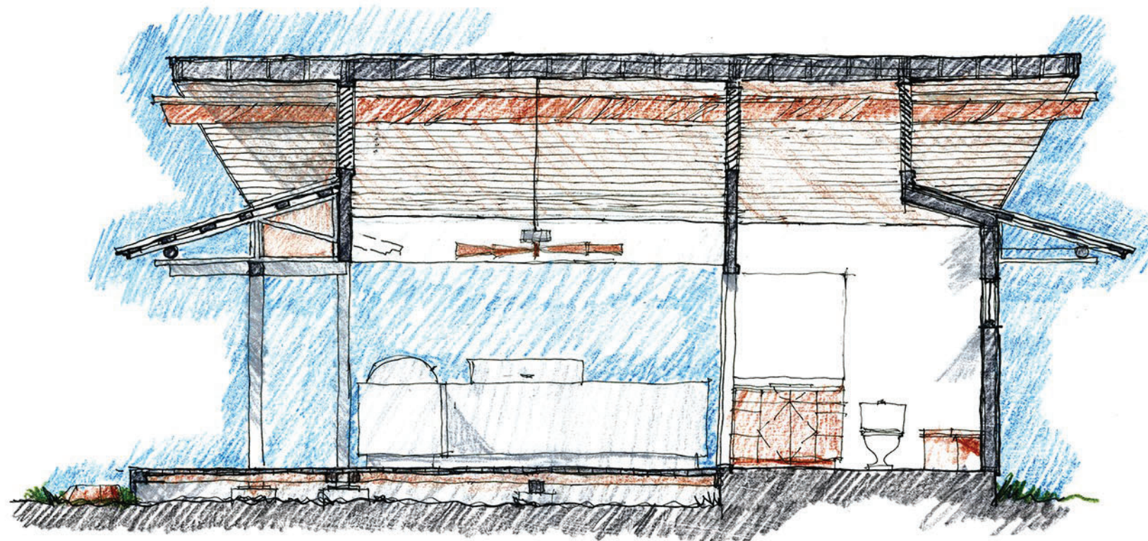
BUILDING SECT # A-A @ CABANA
