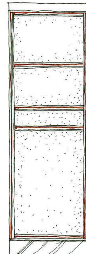
ALTERNATE CONTINUOUS EDGE MUSIC ROOM - RECESS DESIGN REAR VIEW OF SLIDING PANEL
