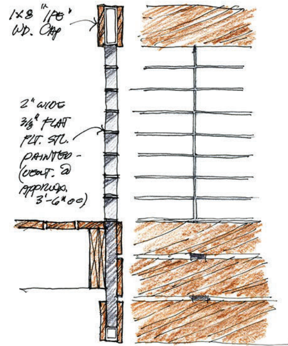
GUARDRAIL #1
